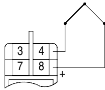
Internal CJC-compensation
