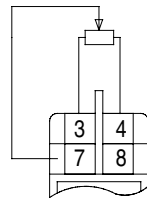
3-wire compensation for transfer resistance {4}
