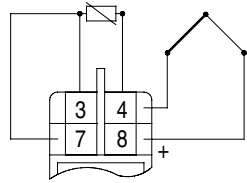
External CJC-compensation 3-wire cable compensation
