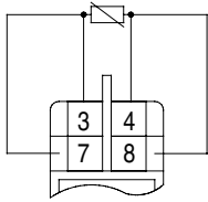
4-wire cable-compensation
