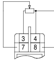
4-wire compensation for transfer resistance {4}
