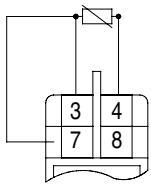
3-wire cable-compensation
