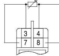
4-wire cable compensation
